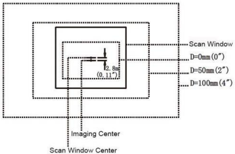
Figure 2-4 Field of view - Front view
