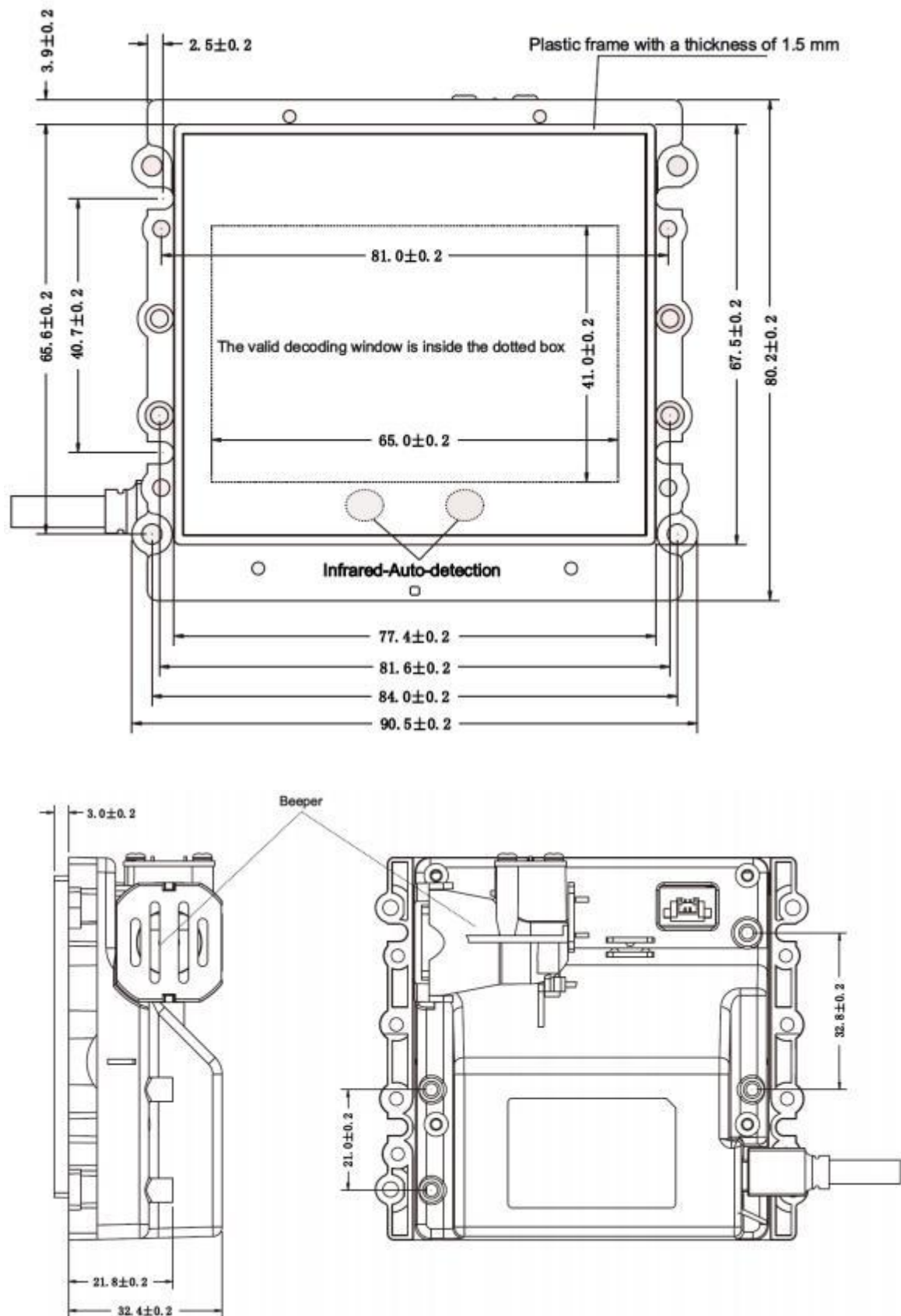
Figure 2-2 Dimensions
